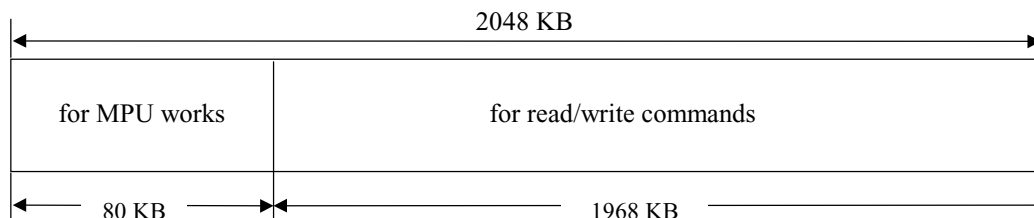
Figure 6.7 Data buffer configuration
