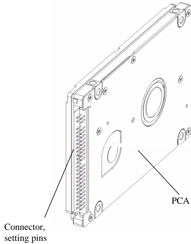
Figure 3.8 Connector locations
