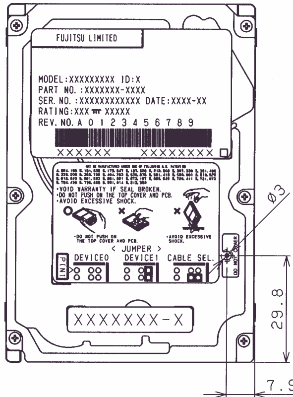
Figure 3.4 Location of breather
