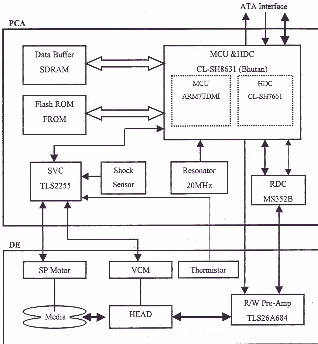
Figure 4.3 Circuit Configuration
