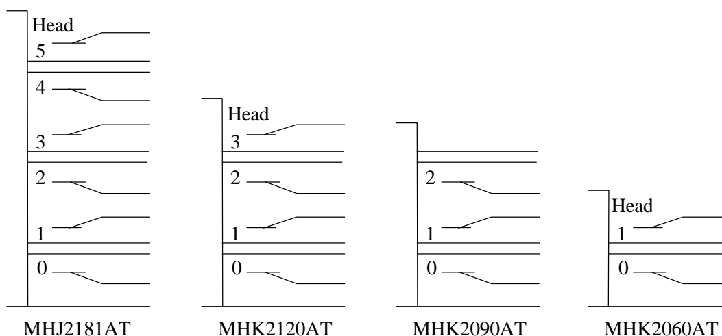
Figure 4.1 Head structure
